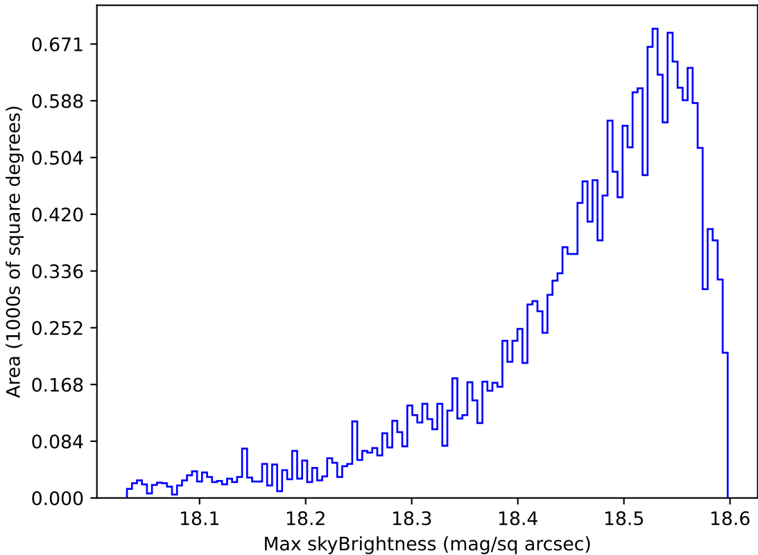
too_elab_r8_d2_ugrizy_v3.4_10yrs Yr 1 y band: Max skyBrightness
