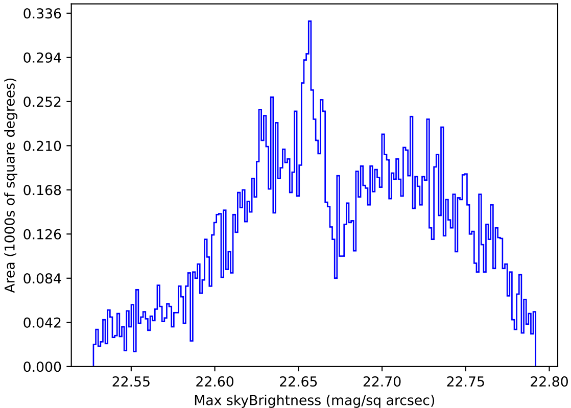
too_elab_r8_d2_ugrizy_v3.4_10yrs Yr 1 u band: Max skyBrightness
