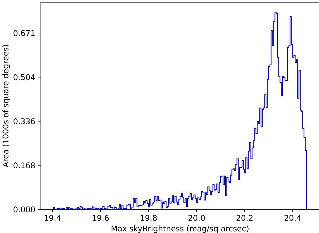
too_elab_r8_d2_ugrizy_v3.4_10yrs Yr 1 i band: Max skyBrightness
