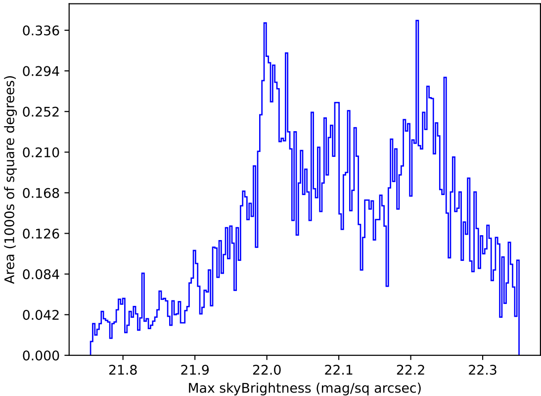
too_elab_r8_d2_ugrizy_v3.4_10yrs Yr 1 g band: Max skyBrightness
