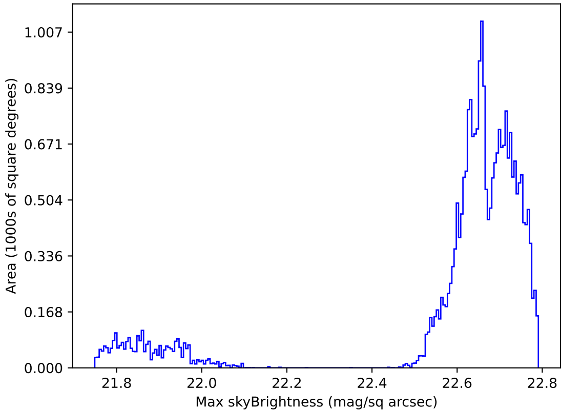
too_elab_r8_d2_ugrizy_v3.4_10yrs Yr 1 all bands: Max skyBrightness
