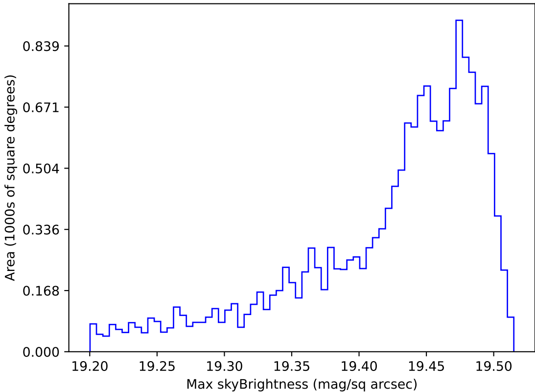
too_elab_r8_d2_ugrizy_v3.4_10yrs WFD z band: Max skyBrightness
