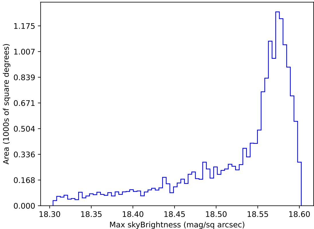
too_elab_r8_d2_ugrizy_v3.4_10yrs WFD y band: Max skyBrightness
