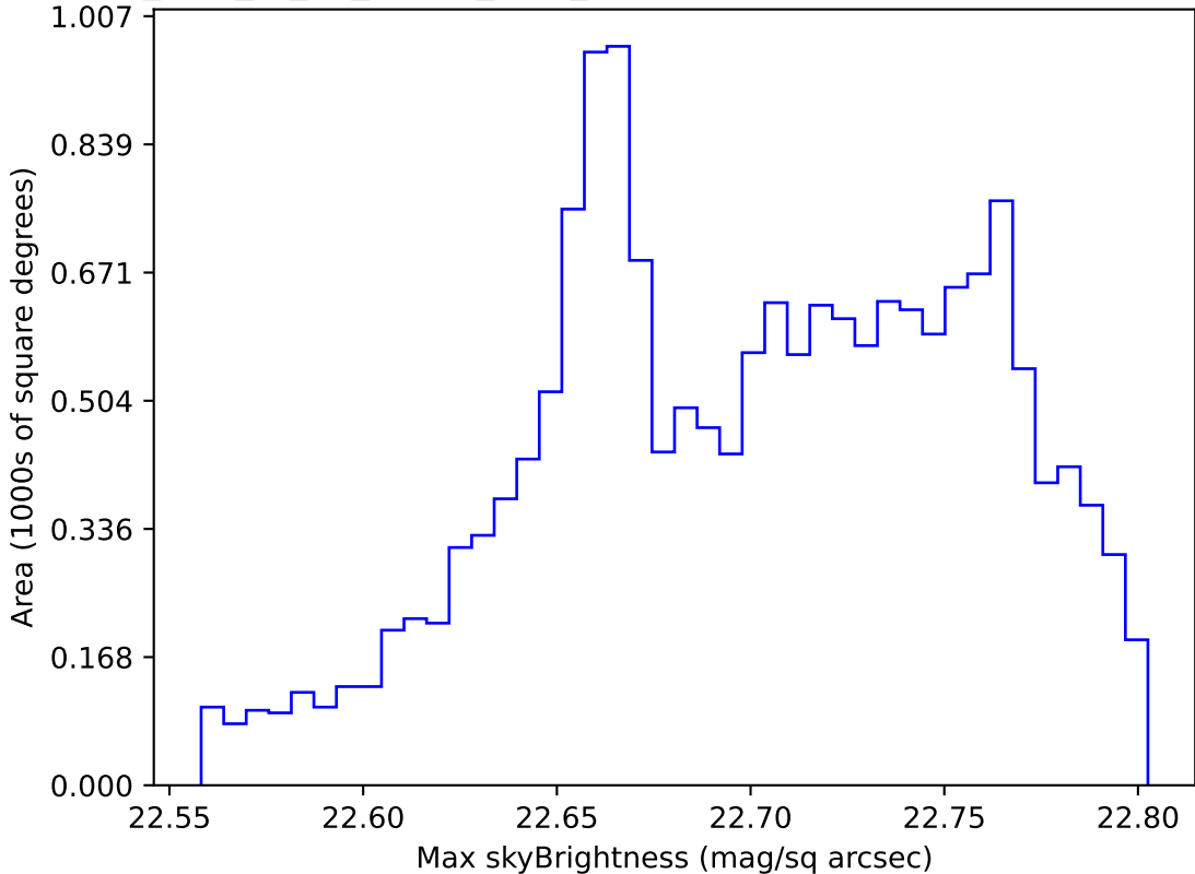
too_elab_r8_d2_ugrizy_v3.4_10yrs WFD u band: Max skyBrightness
