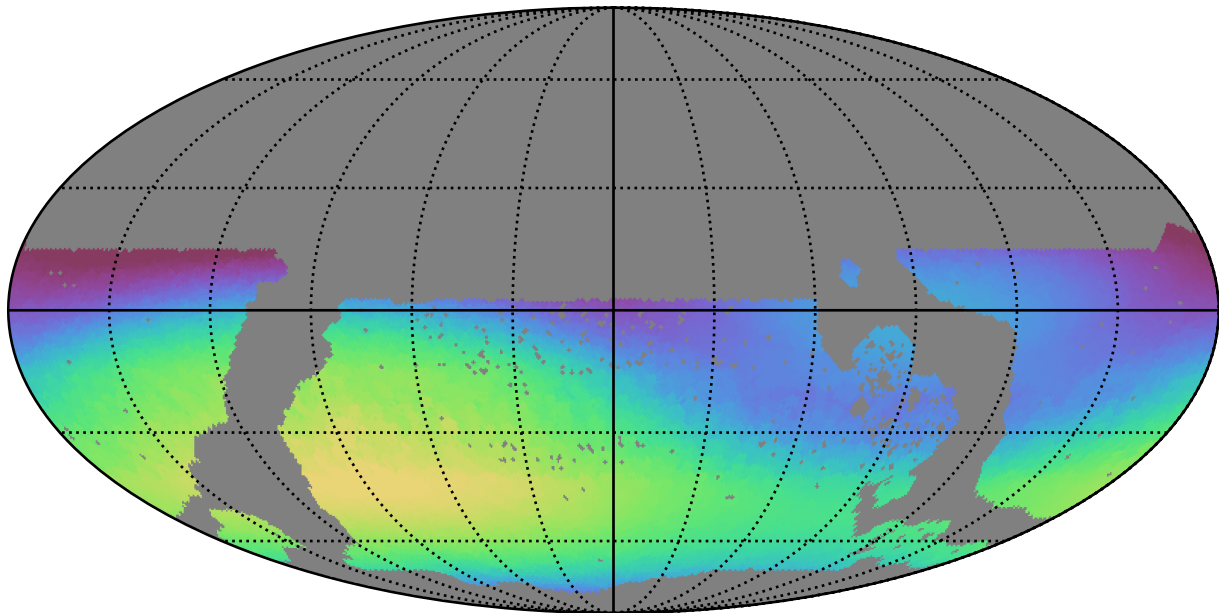
too_elab_r8_d2_ugrizy_v3.4_10yrs WFD r band: Max skyBrightness
