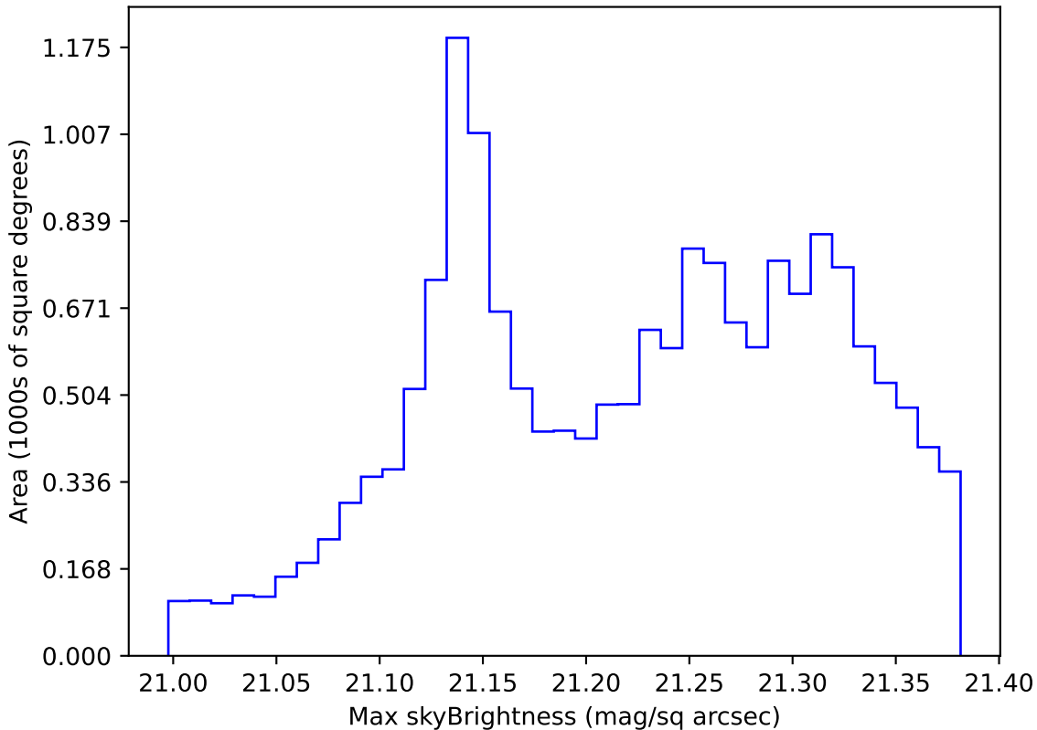
too_elab_r8_d2_ugrizy_v3.4_10yrs WFD r band: Max skyBrightness
