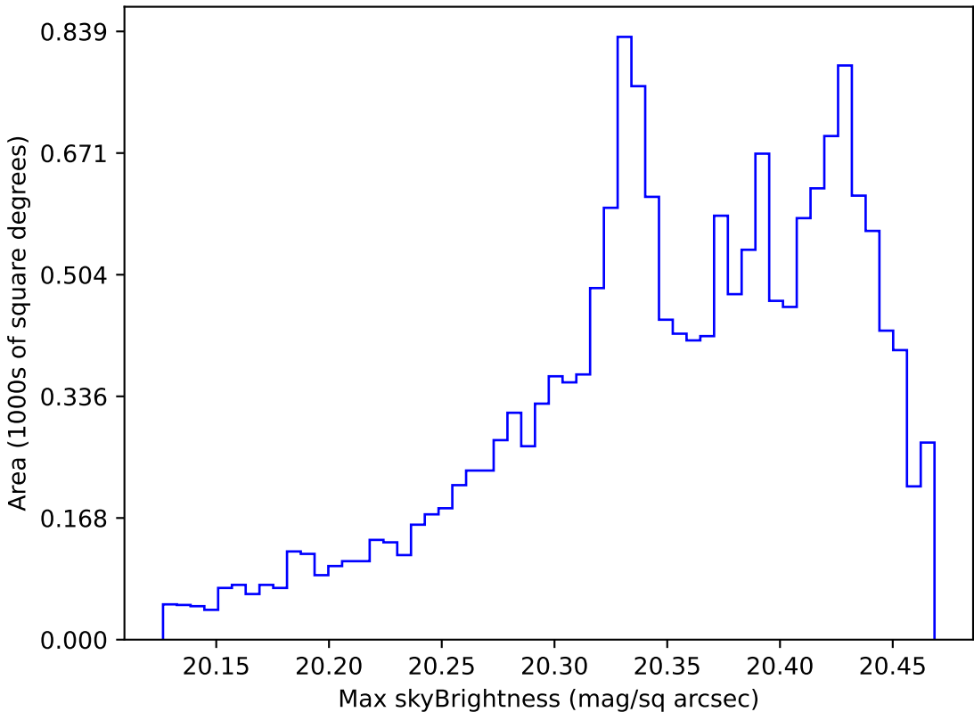
too_elab_r8_d2_ugrizy_v3.4_10yrs WFD i band: Max skyBrightness
