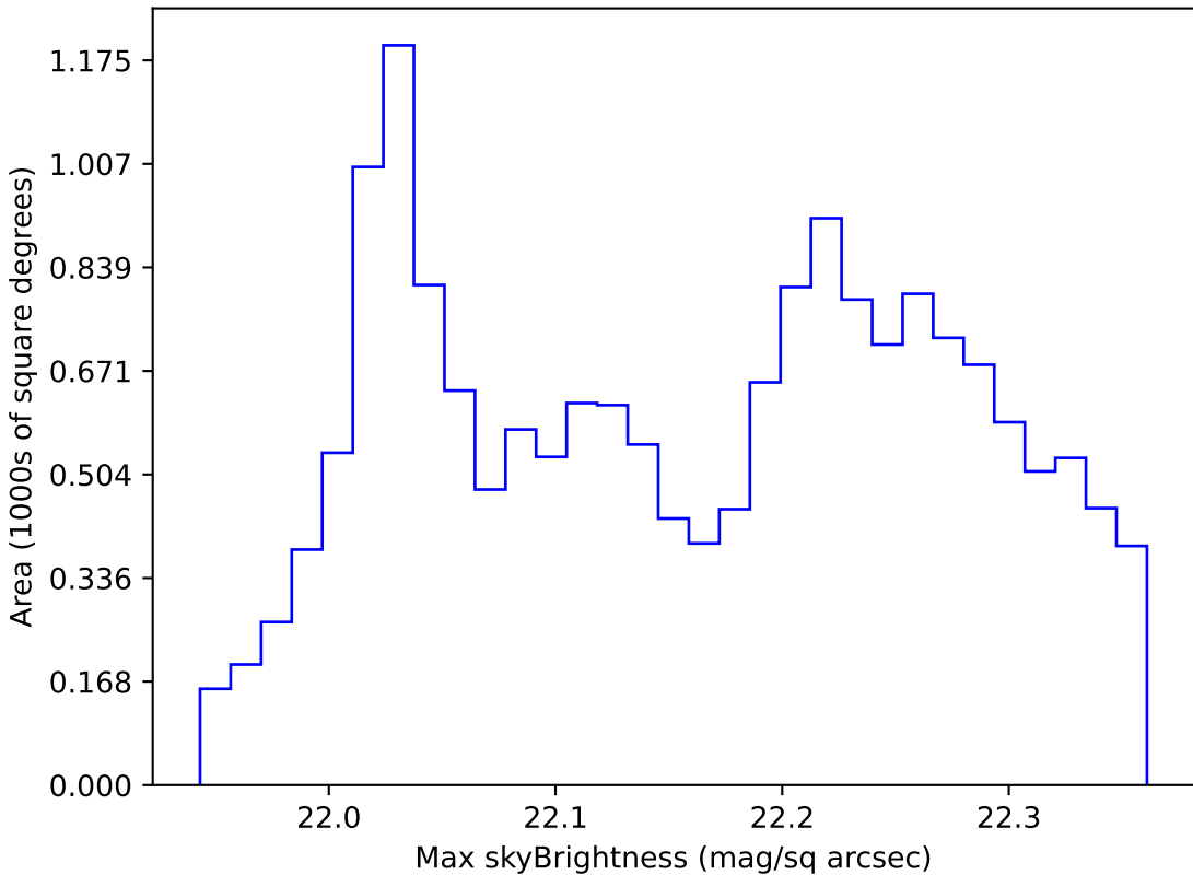
too_elab_r8_d2_ugrizy_v3.4_10yrs WFD g band: Max skyBrightness
