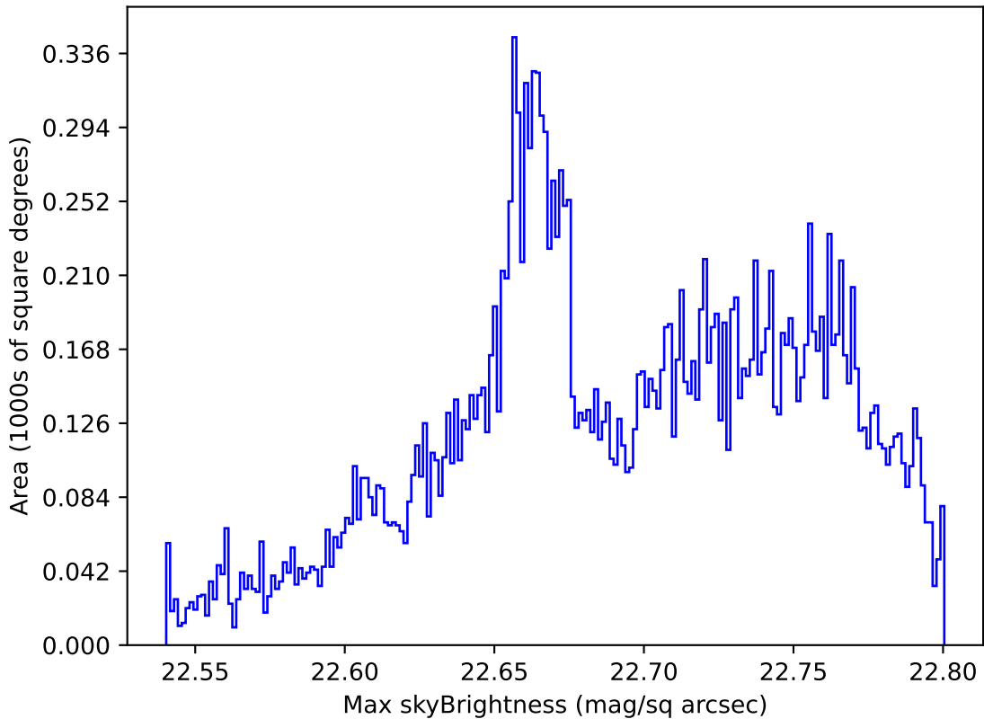
too_elab_r8_d2_ugrizy_v3.4_10yrs All sky u band: Max skyBrightness
