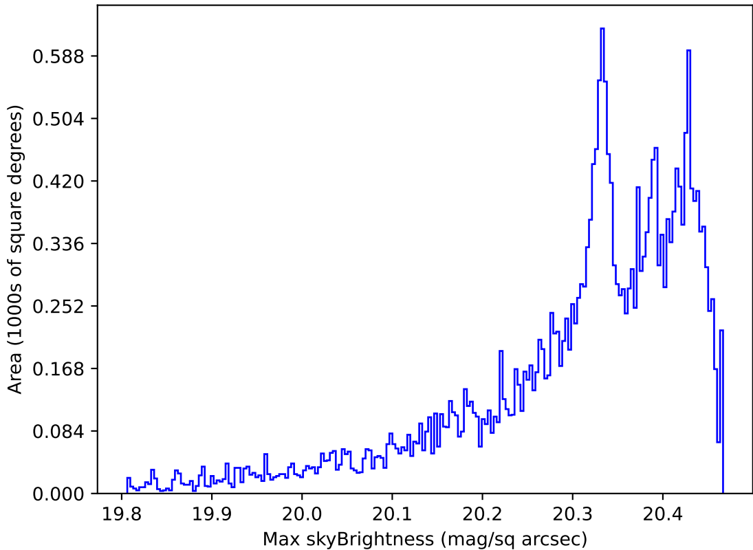
too_elab_r8_d2_ugrizy_v3.4_10yrs All sky i band: Max skyBrightness
