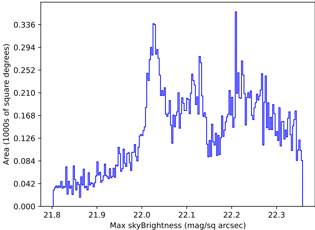
too_elab_r8_d2_ugrizy_v3.4_10yrs All sky g band: Max skyBrightness
