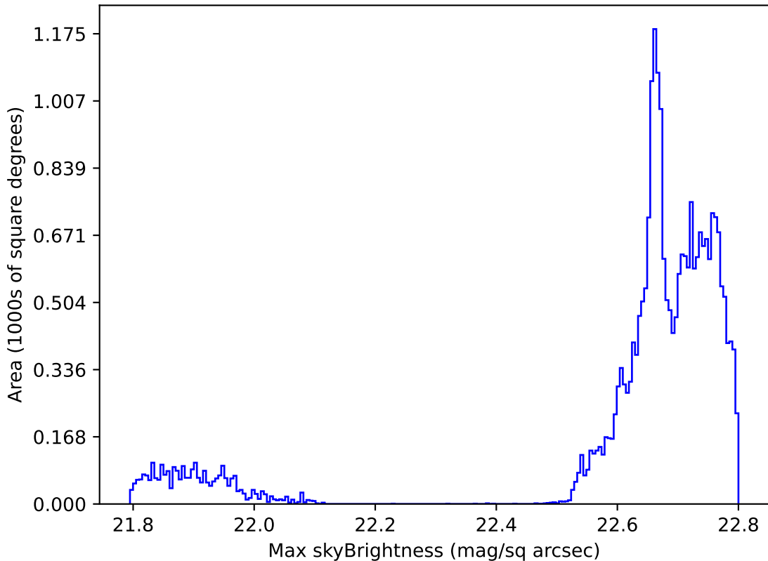
too_elab_r8_d2_ugrizy_v3.4_10yrs All sky all bands: Max skyBrightness
