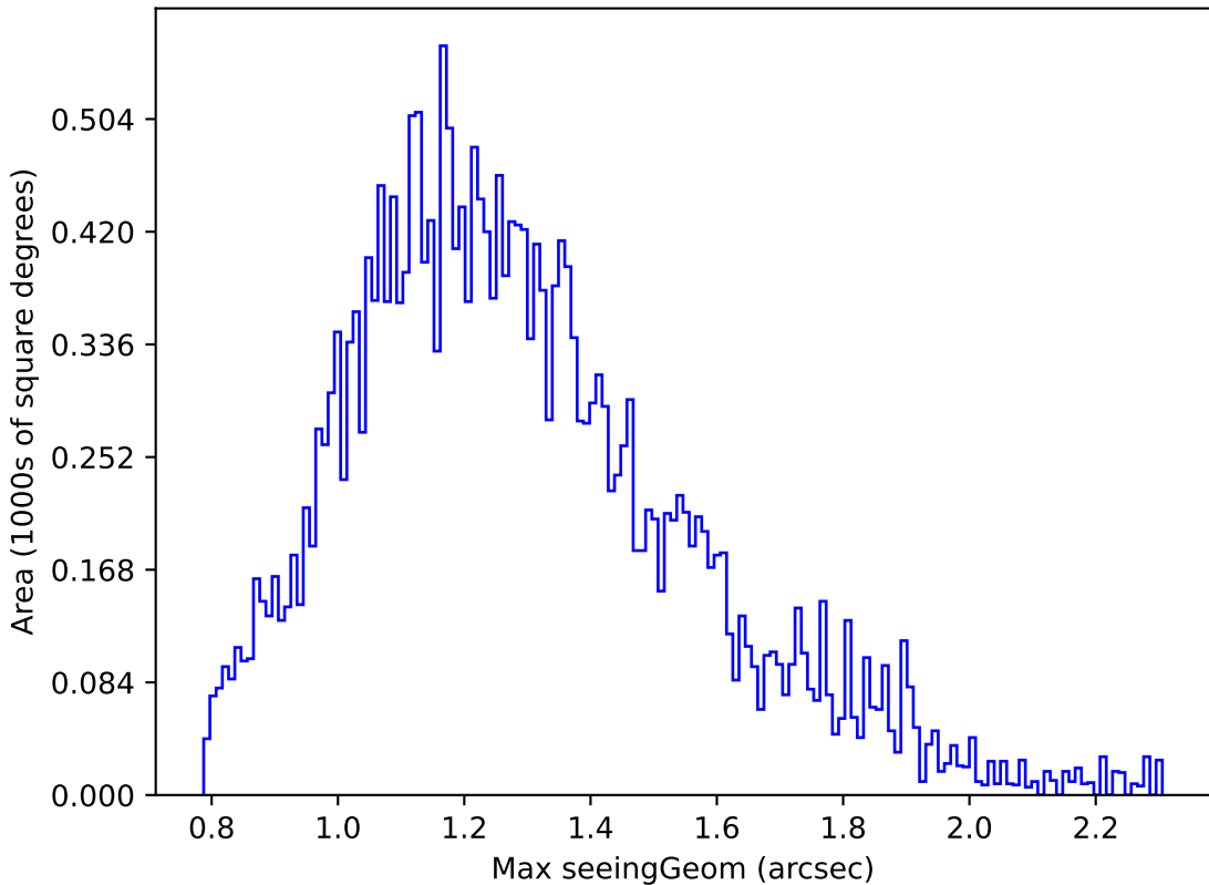
too_elab_r8_d2_ugrizy_v3.4_10yrs Yr 1 z band: Max seeingGeom
