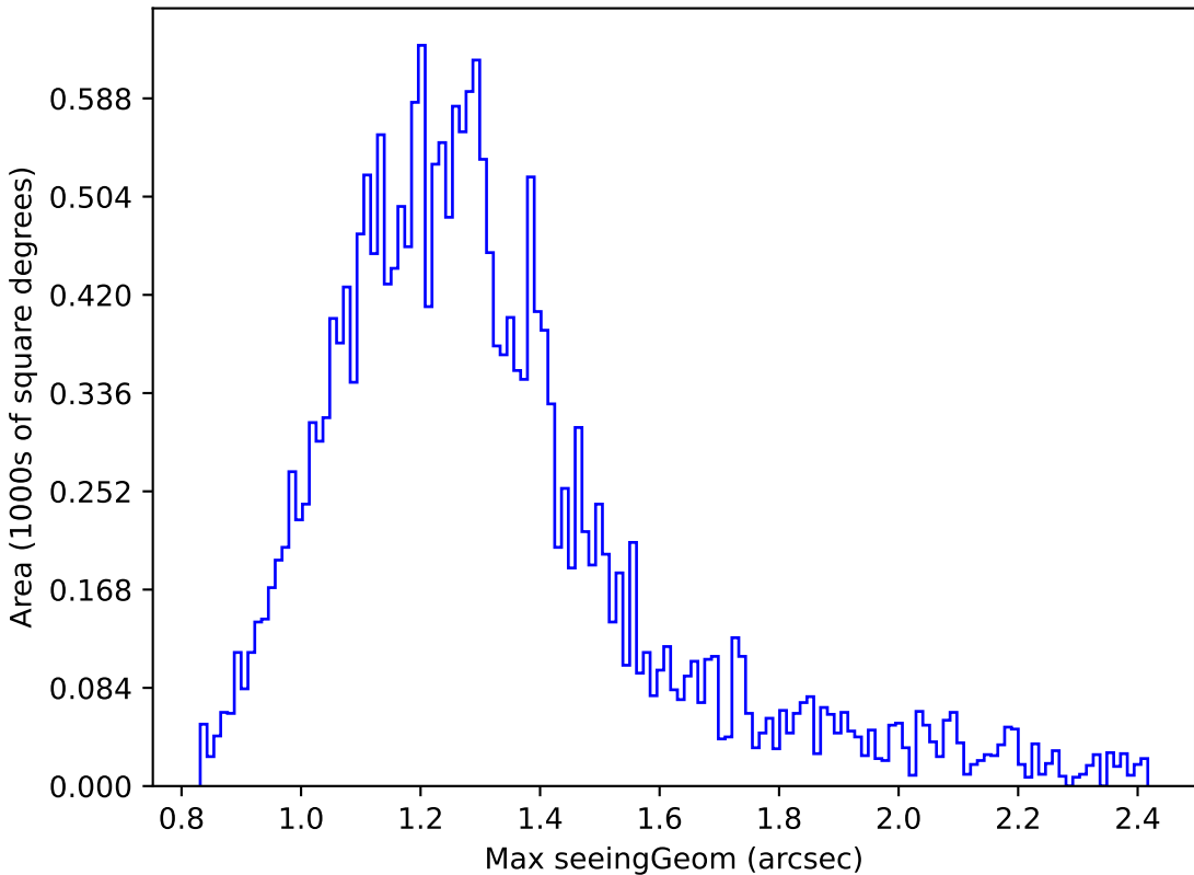
too_elab_r8_d2_ugrizy_v3.4_10yrs Yr 1 y band: Max seeingGeom
