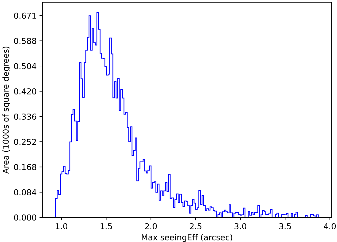
too_elab_r8_d2_ugrizy_v3.4_10yrs Yr 1 u band: Max seeingEff
