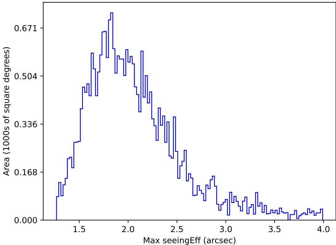
too_elab_r8_d2_ugrizy_v3.4_10yrs Yr 1 all bands: Max seeingEff
