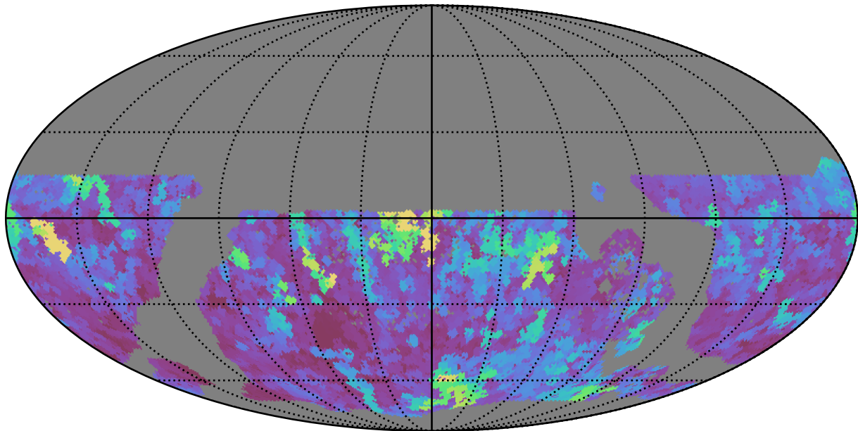
too_elab_r8_d2_ugrizy_v3.4_10yrs WFD z band: Max seeingEff
