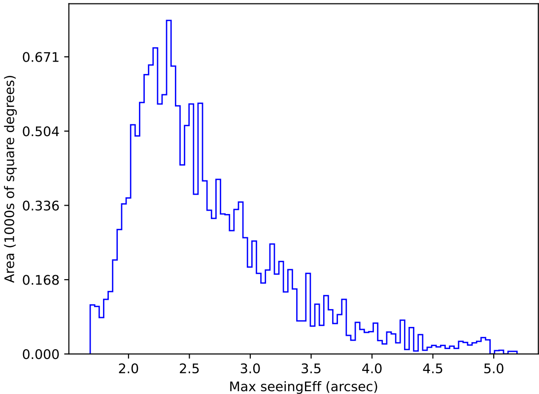
too_elab_r8_d2_ugrizy_v3.4_10yrs WFD z band: Max seeingEff
