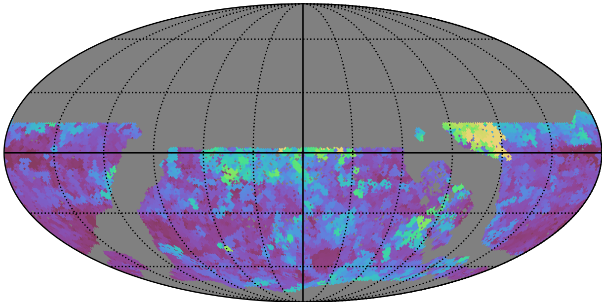
too_elab_r8_d2_ugrizy_v3.4_10yrs WFD u band: Max seeingEff
