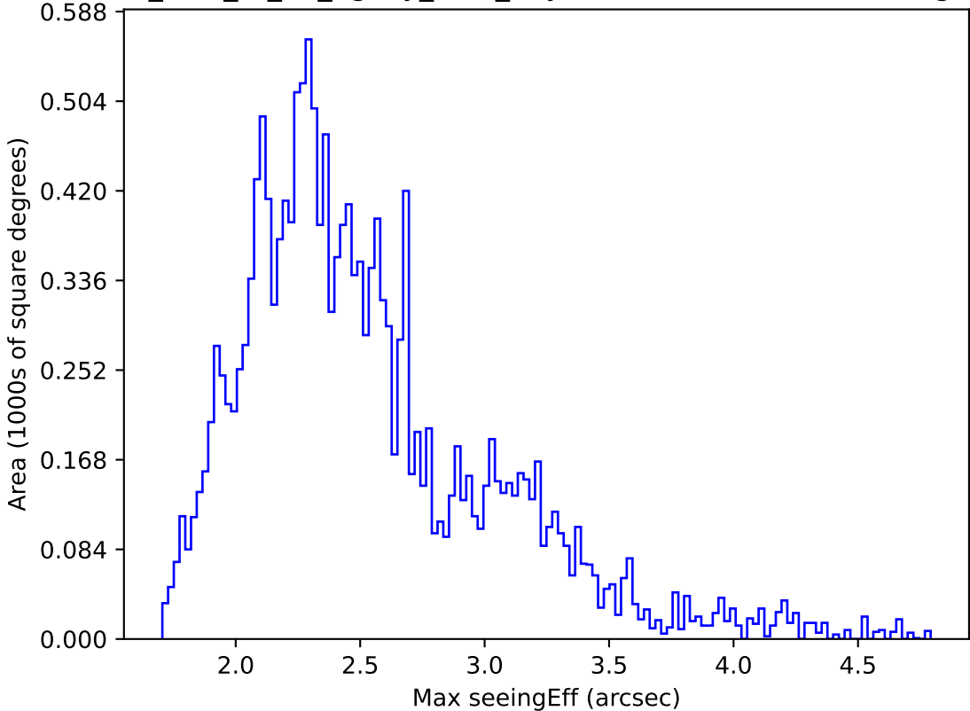
too_elab_r8_d2_ugrizy_v3.4_10yrs WFD u band: Max seeingEff
