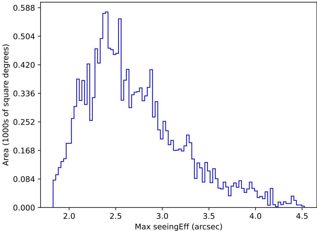
too_elab_r8_d2_ugrizy_v3.4_10yrs WFD r band: Max seeingEff
