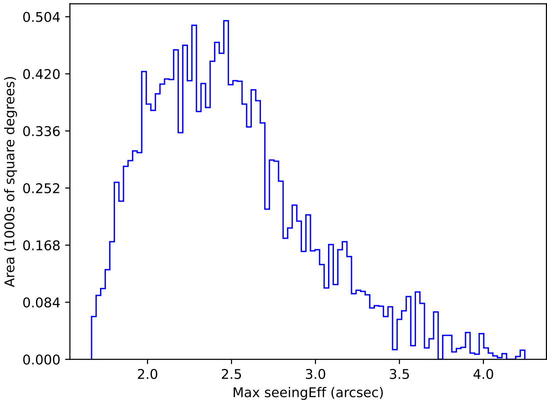
too_elab_r8_d2_ugrizy_v3.4_10yrs WFD g band: Max seeingEff
