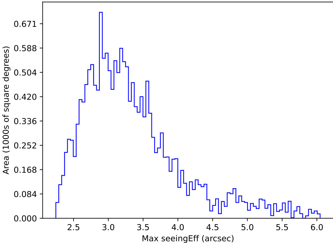
too_elab_r8_d2_ugrizy_v3.4_10yrs WFD all bands: Max seeingEff
