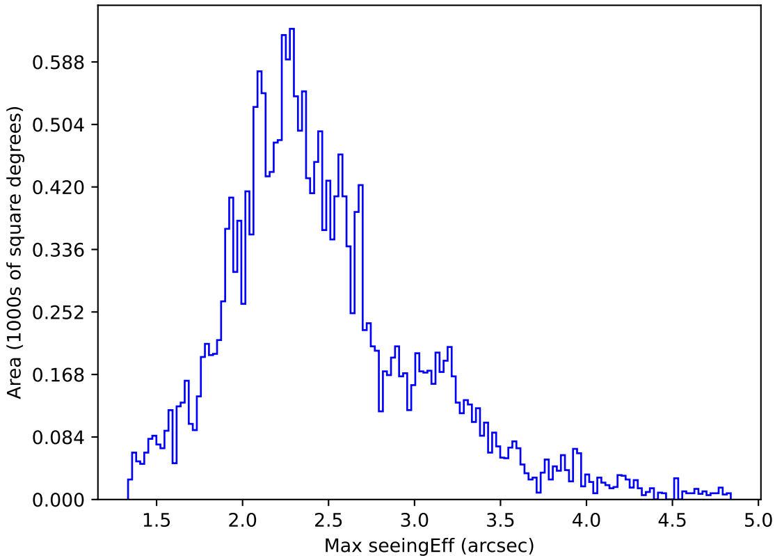
too_elab_r8_d2_ugrizy_v3.4_10yrs All sky u band: Max seeingEff
