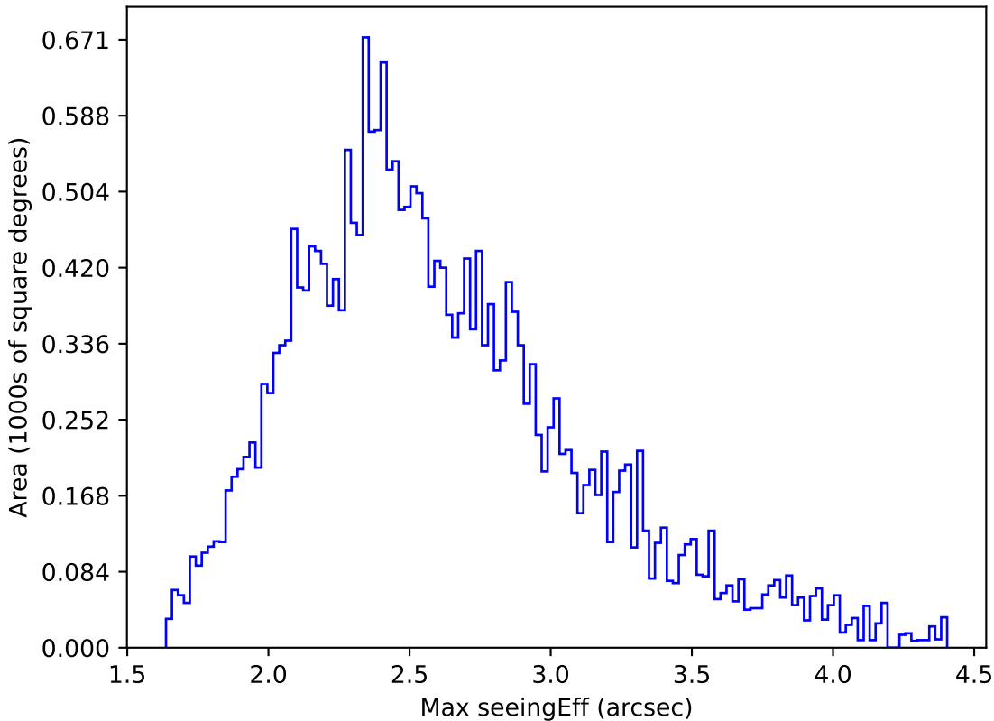
too_elab_r8_d2_ugrizy_v3.4_10yrs All sky r band: Max seeingEff
