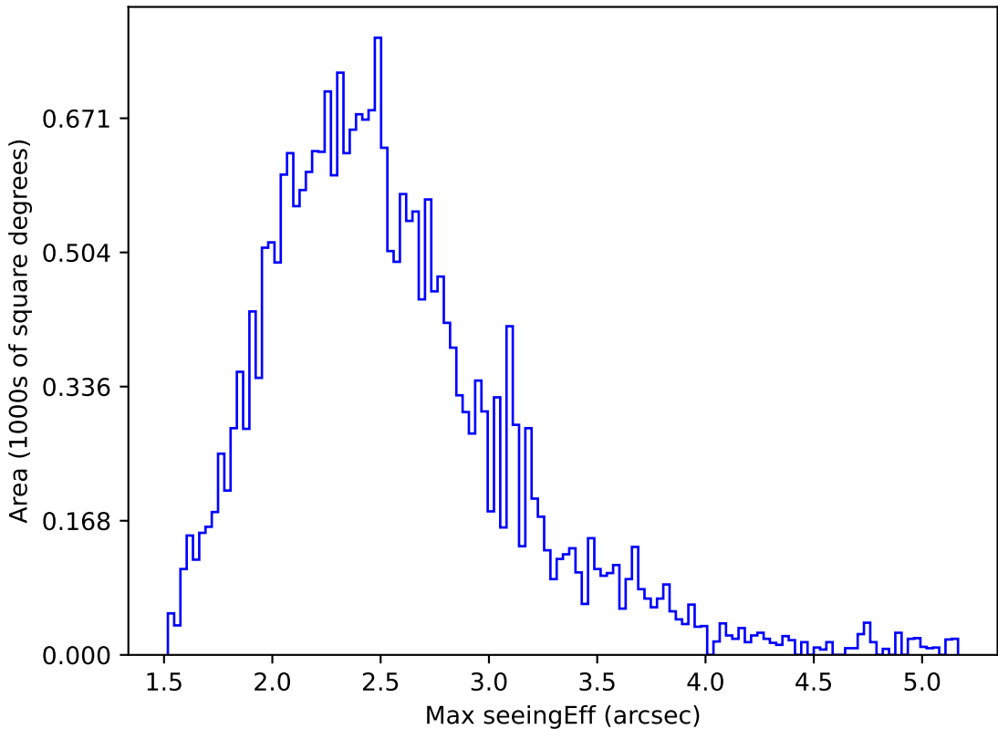
too_elab_r8_d2_ugrizy_v3.4_10yrs All sky i band: Max seeingEff
