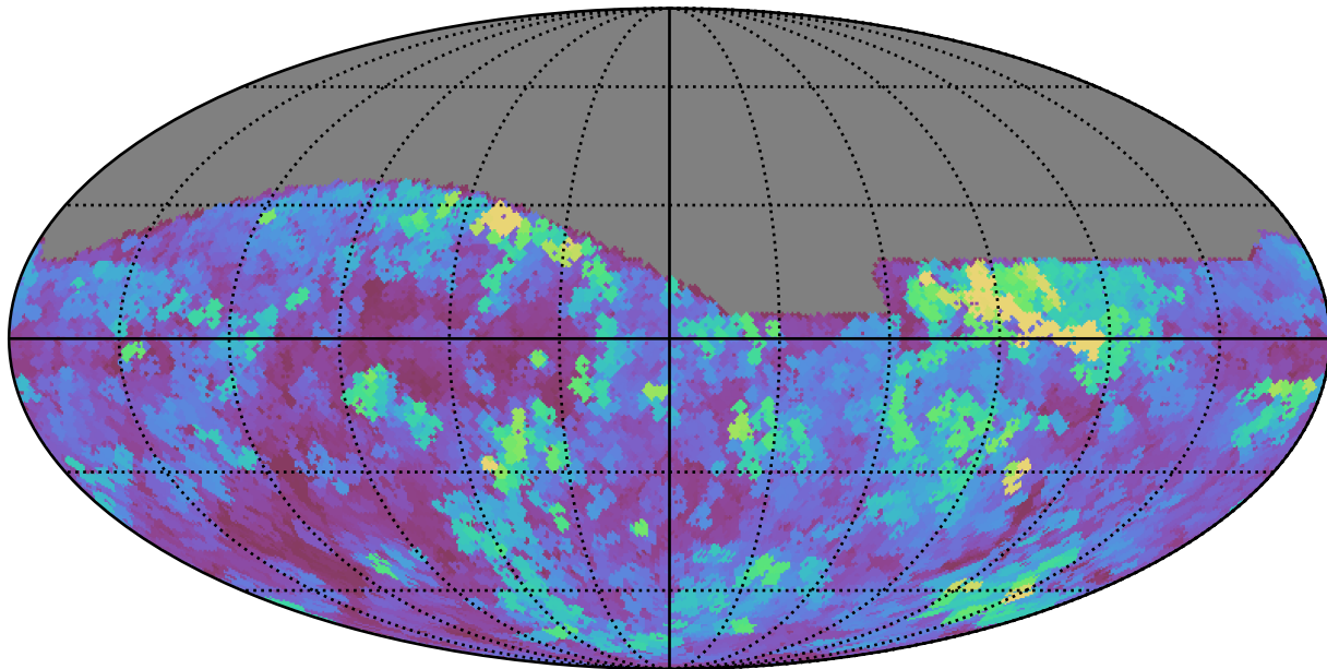
too_elab_r8_d2_ugrizy_v3.4_10yrs All sky g band: Max seeingEff
