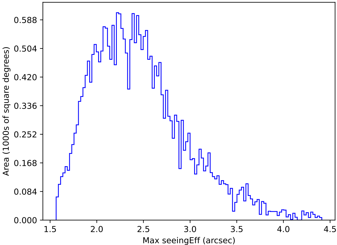
too_elab_r8_d2_ugrizy_v3.4_10yrs All sky g band: Max seeingEff
