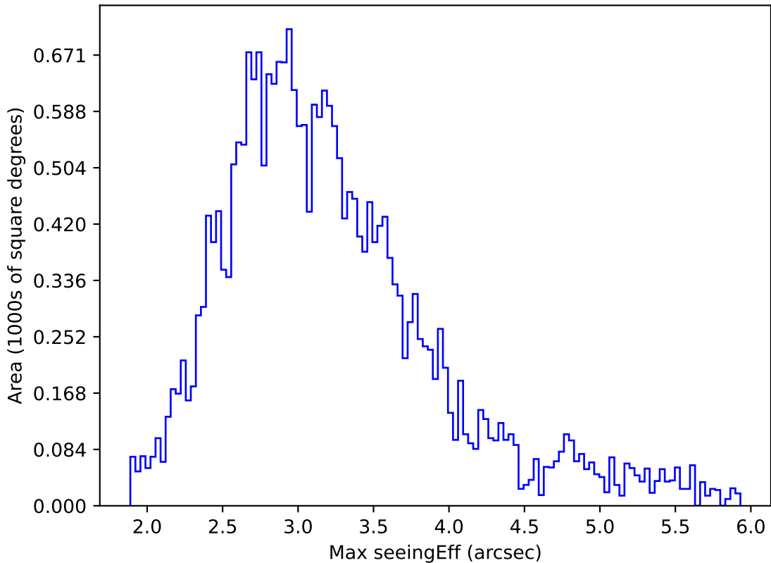
too_elab_r8_d2_ugrizy_v3.4_10yrs All sky all bands: Max seeingEff
