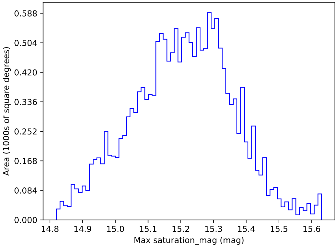
too_elab_r8_d2_ugrizy_v3.4_10yrs WFD z band: Max saturation_mag
