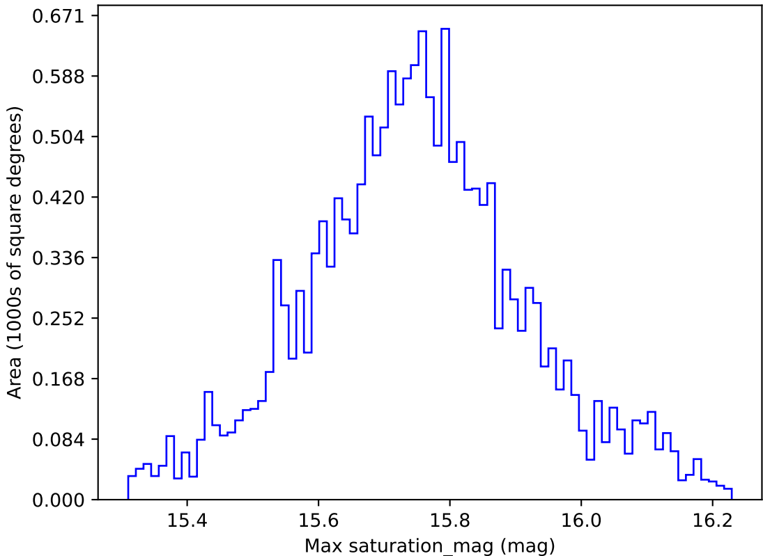
too_elab_r8_d2_ugrizy_v3.4_10yrs WFD r band: Max saturation_mag
