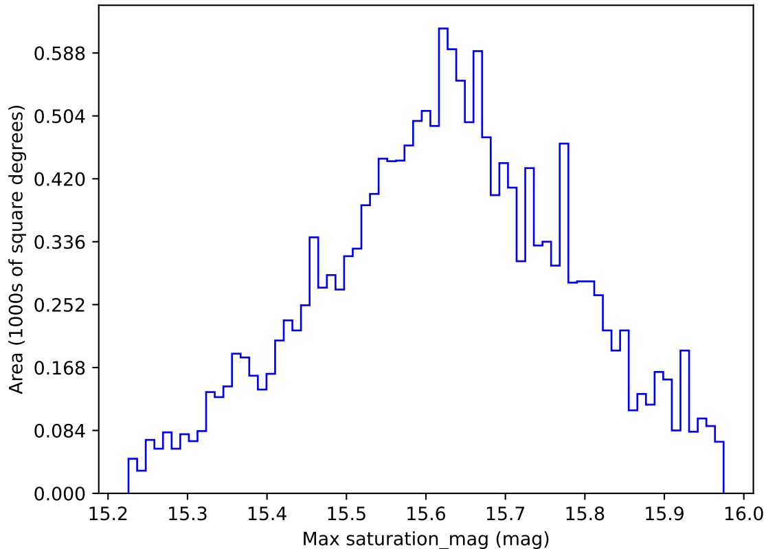
too_elab_r8_d2_ugrizy_v3.4_10yrs WFD i band: Max saturation_mag
