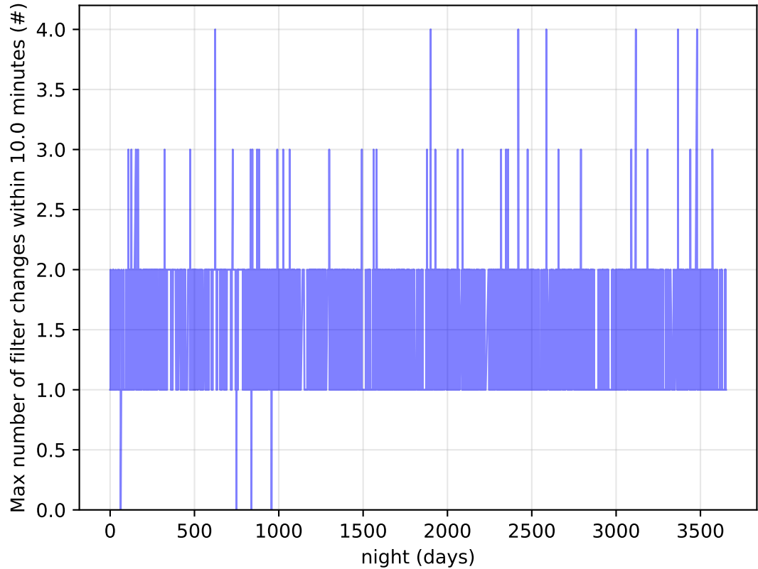
too_elab_r8_d2_ugrizy_v3.4_10yrs Per Night: Max number of filter changes within 10.0 minutes
