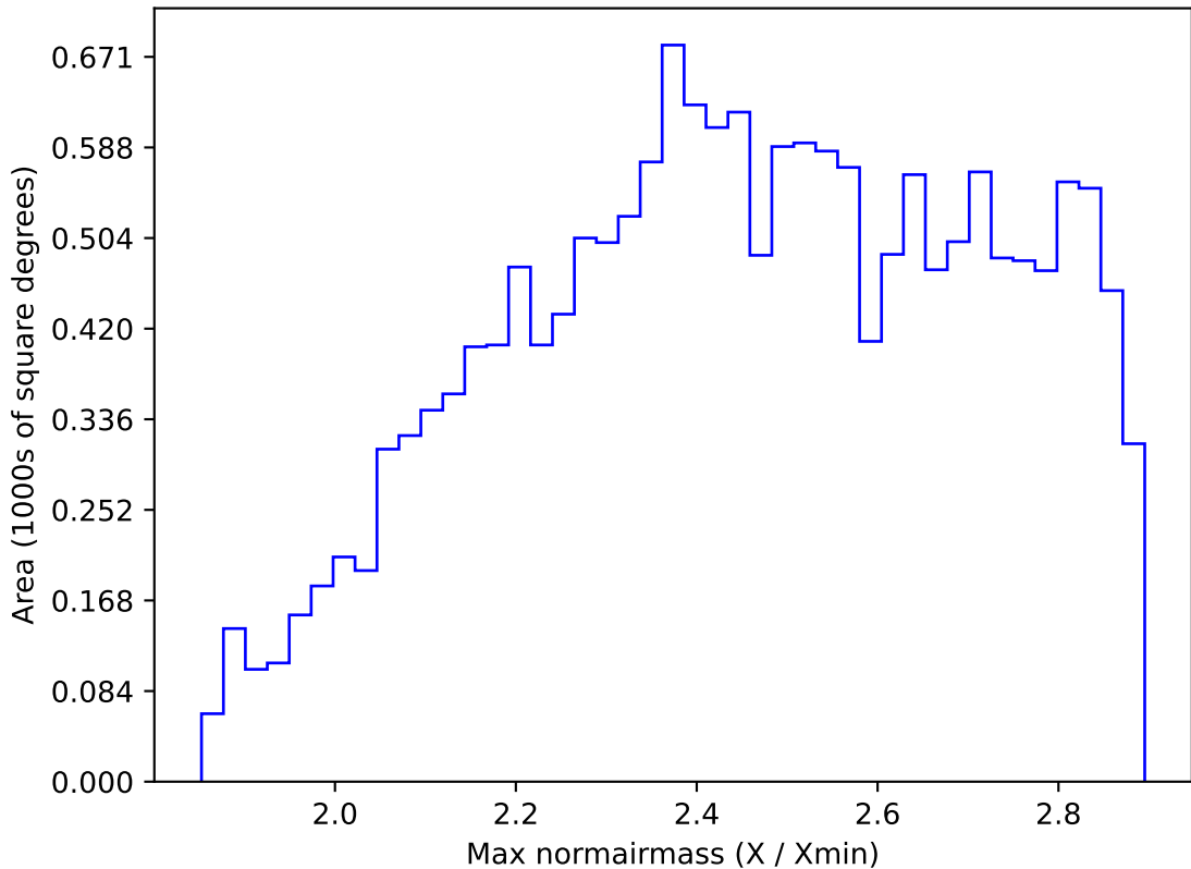
too_elab_r8_d2_ugrizy_v3.4_10yrs WFD all bands: Max normairmass
