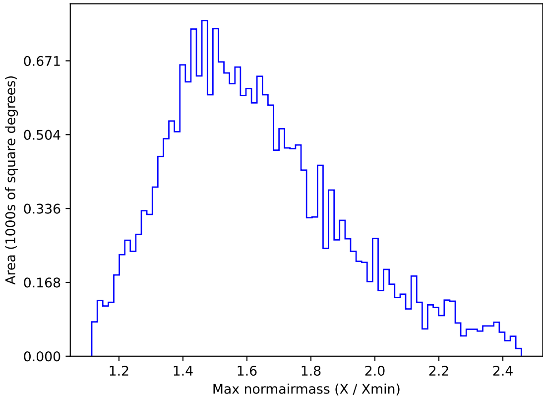
too_elab_r8_d2_ugrizy_v3.4_10yrs All sky u band: Max normairmass
