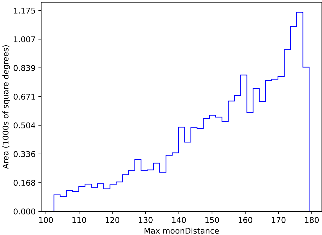
too_elab_r8_d2_ugrizy_v3.4_10yrs WFD z band: Max moonDistance
