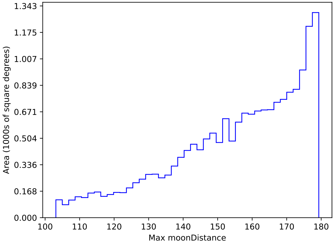
too_elab_r8_d2_ugrizy_v3.4_10yrs WFD i band: Max moonDistance
