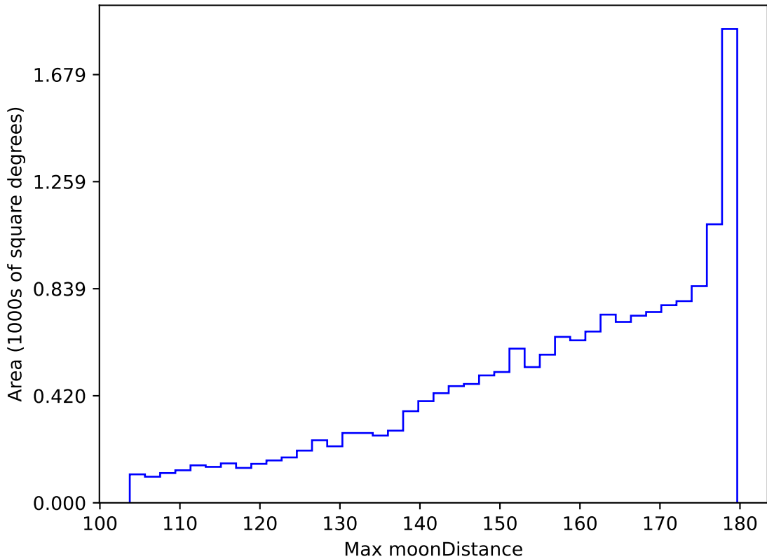
too_elab_r8_d2_ugrizy_v3.4_10yrs WFD all bands: Max moonDistance
