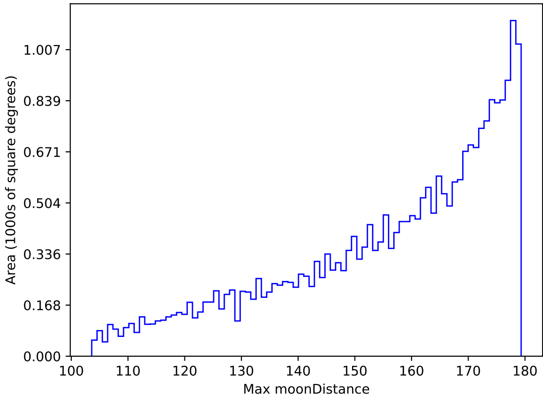
too_elab_r8_d2_ugrizy_v3.4_10yrs All sky r band: Max moonDistance
