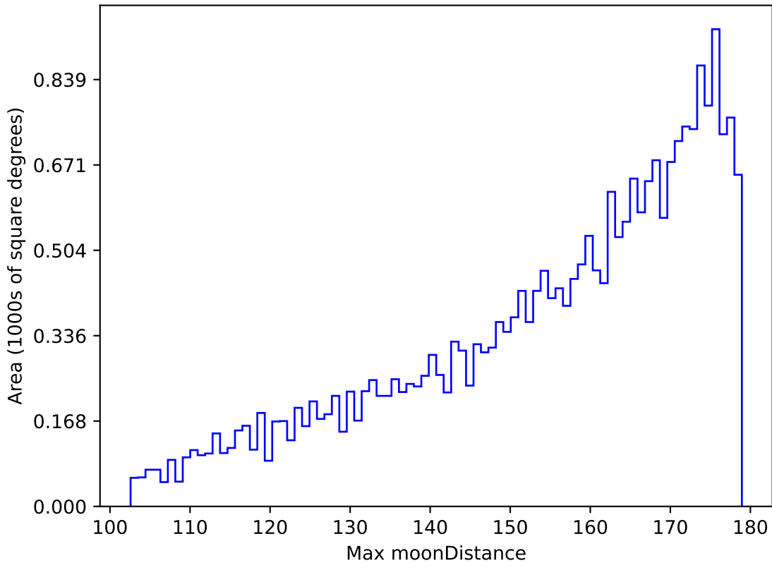
too_elab_r8_d2_ugrizy_v3.4_10yrs All sky g band: Max moonDistance
