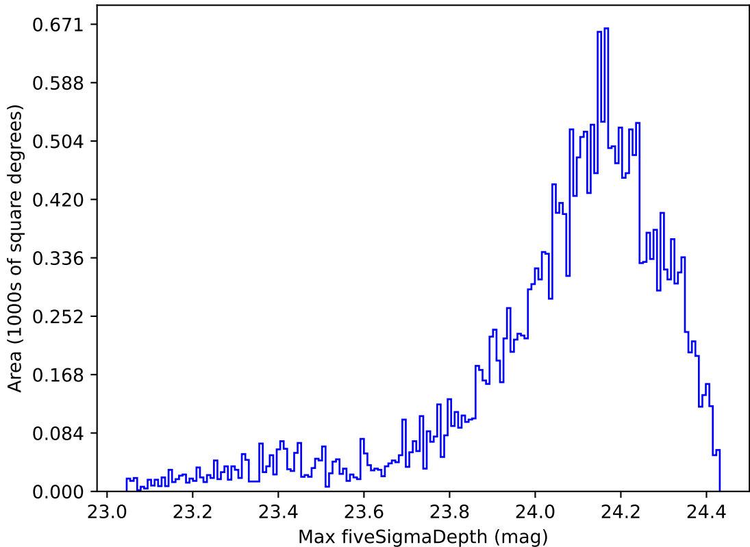
too_elab_r8_d2_ugrizy_v3.4_10yrs Yr 1 i band: Max fiveSigmaDepth
