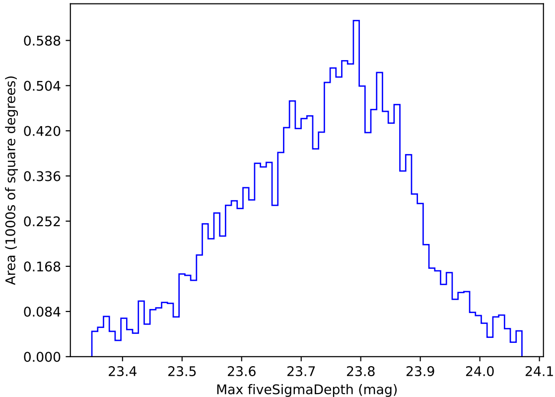
too_elab_r8_d2_ugrizy_v3.4_10yrs WFD u band: Max fiveSigmaDepth
