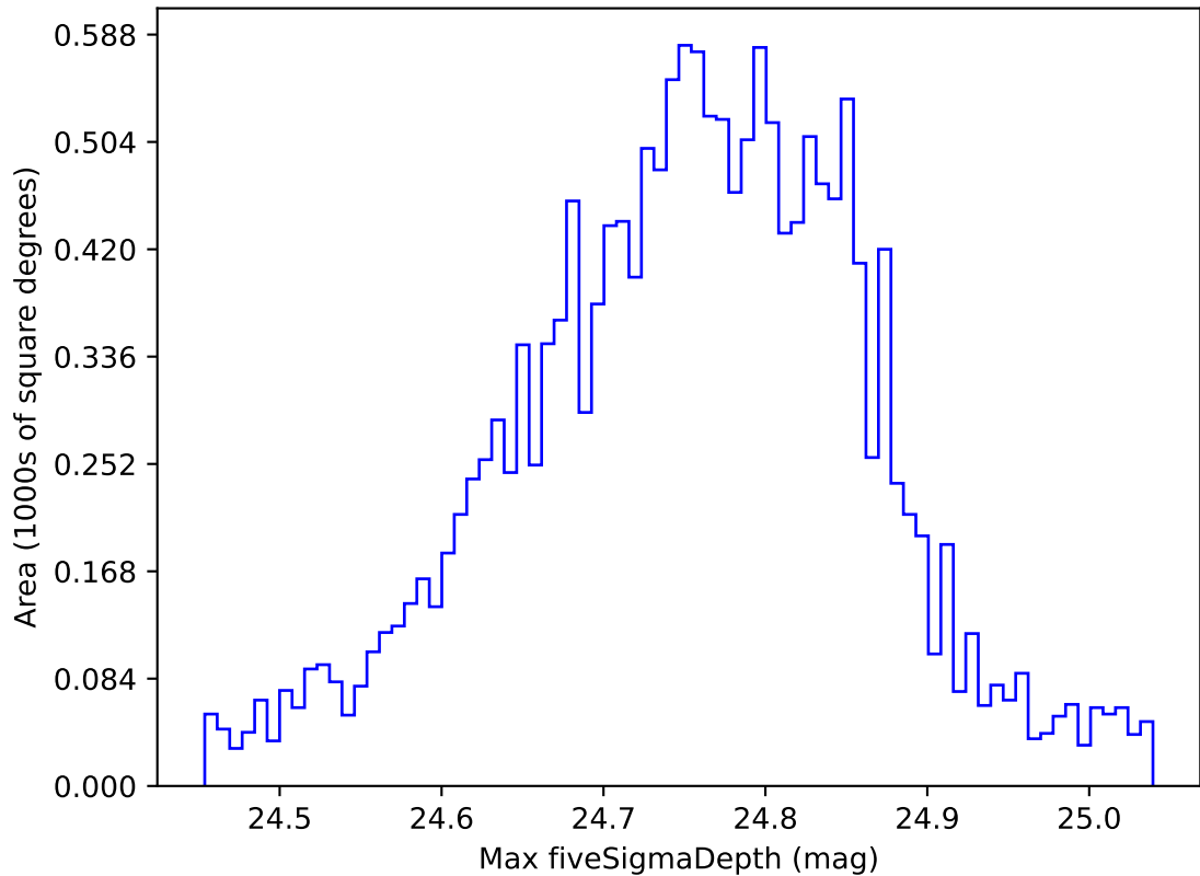
too_elab_r8_d2_ugrizy_v3.4_10yrs WFD r band: Max fiveSigmaDepth
