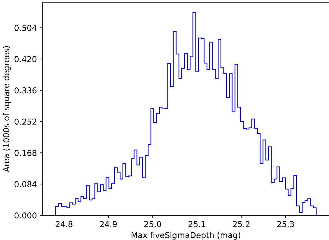
too_elab_r8_d2_ugrizy_v3.4_10yrs WFD g band: Max fiveSigmaDepth
