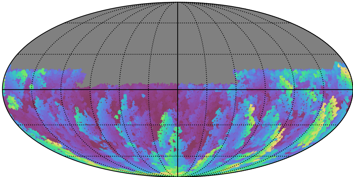
too_elab_r8_d2_ugrizy_v3.4_10yrs Yr 1 u band: Max airmass
