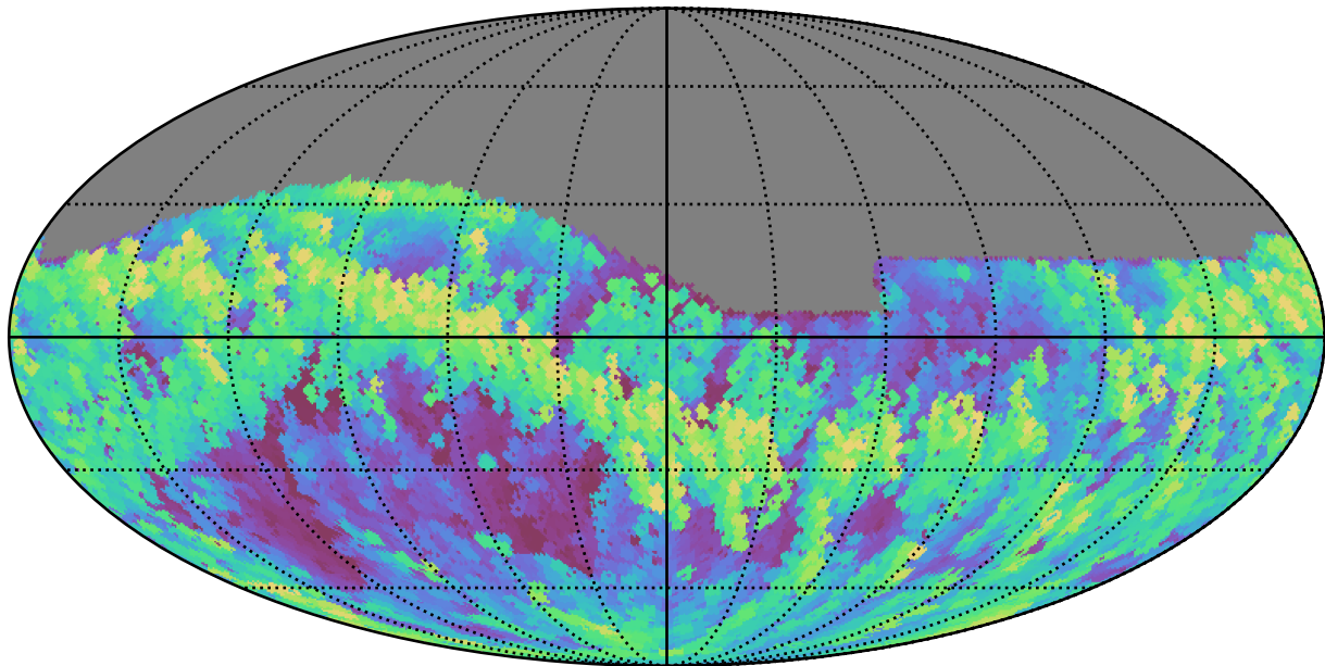
too_elab_r8_d2_ugrizy_v3.4_10yrs Yr 1 all bands: Max airmass
